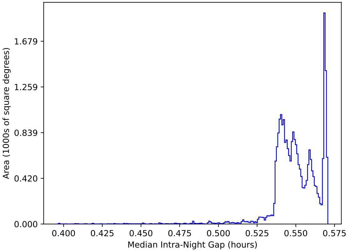
too_ignore_10_1v3.4_10yrs All sky: Median Intra-Night Gap
