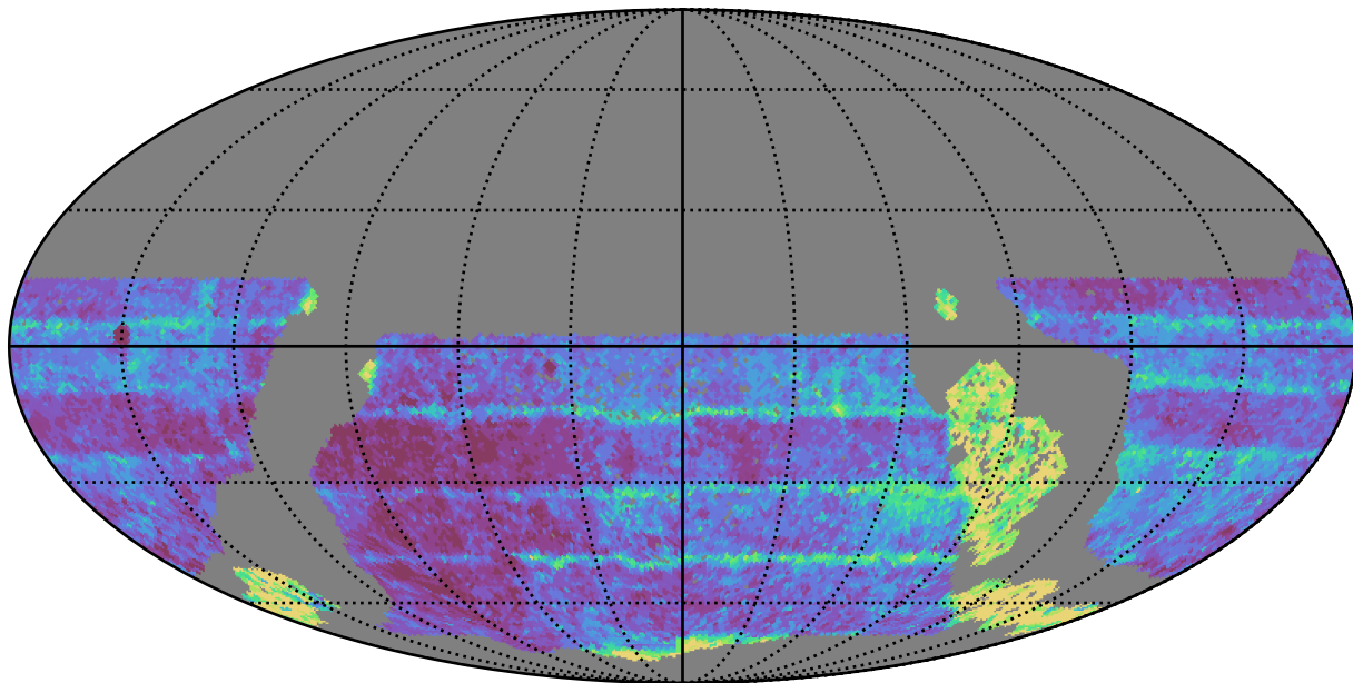
too_ignore_10_1v3.4_10yrs WFD z band: Median Inter-Night Gap
