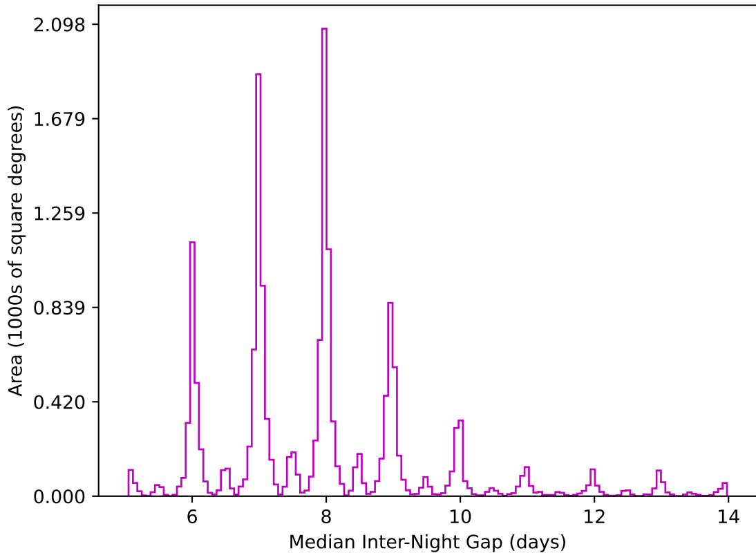
too_ignore_10_1v3.4_10yrs WFD z band: Median Inter-Night Gap
