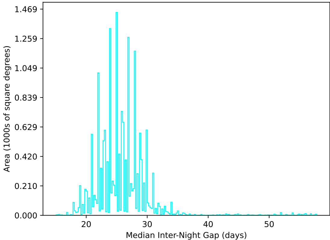
too_ignore_10_1v3.4_10yrs WFD u band: Median Inter-Night Gap
