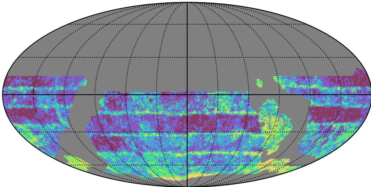
too_ignore_10_1v3.4_10yrs WFD r band: Median Inter-Night Gap
