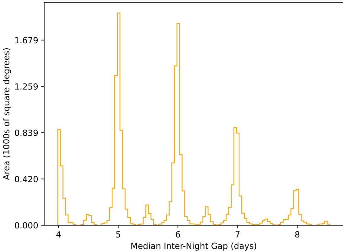
too_ignore_10_1v3.4_10yrs WFD r band: Median Inter-Night Gap
