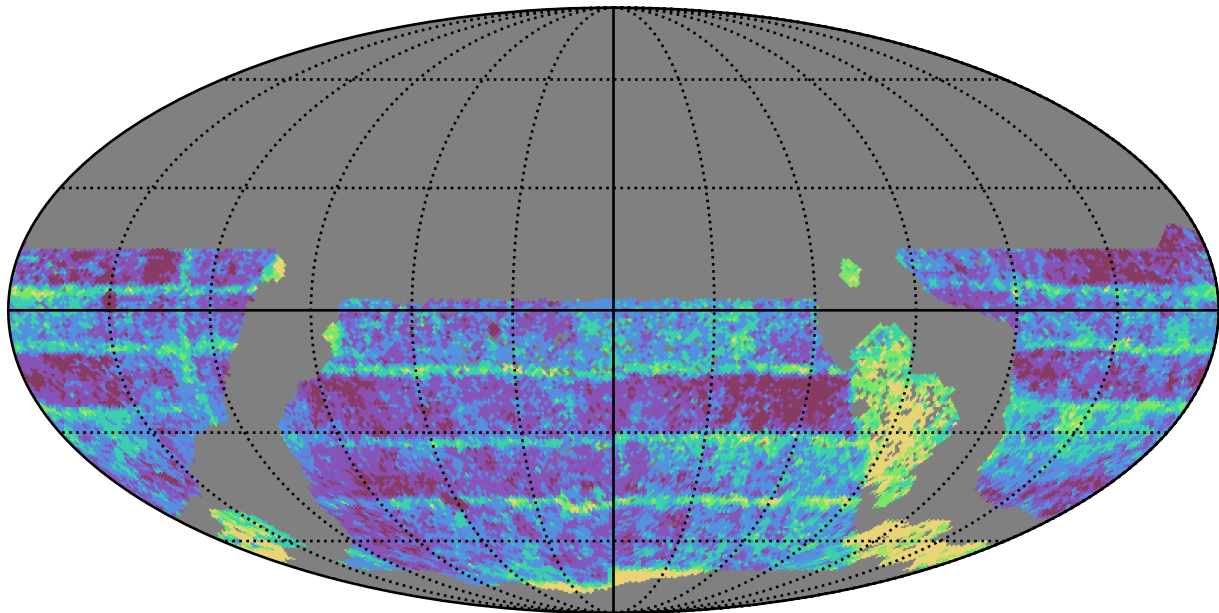
too_ignore_10_1v3.4_10yrs WFD i band: Median Inter-Night Gap
