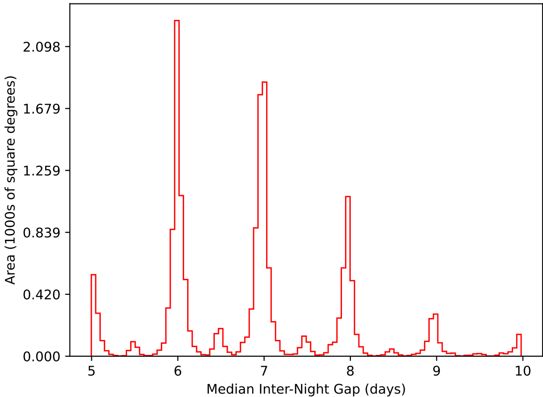
too_ignore_10_1v3.4_10yrs WFD i band: Median Inter-Night Gap
