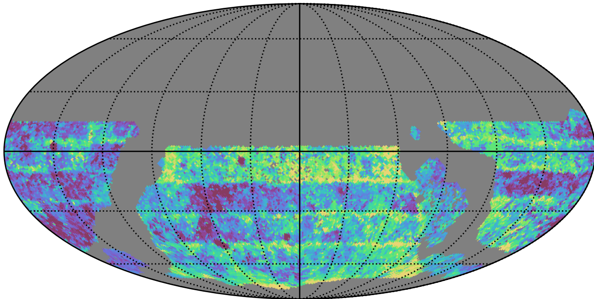
too_ignore_10_1v3.4_10yrs WFD g band: Median Inter-Night Gap
