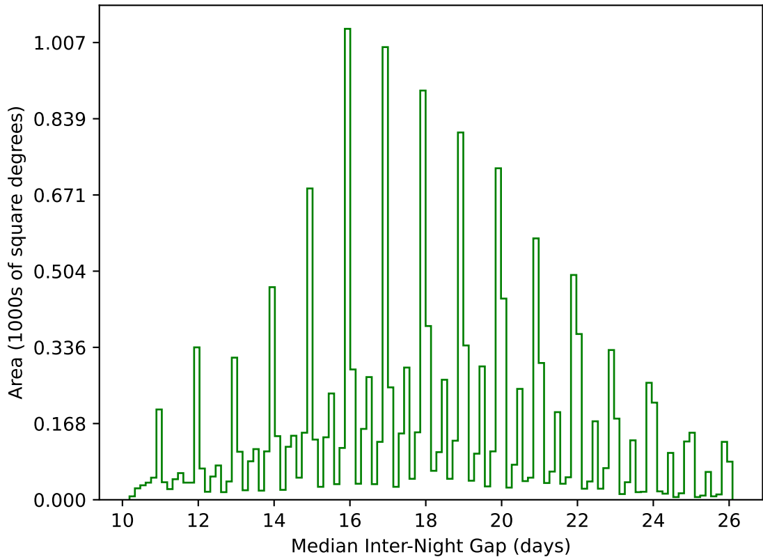
too_ignore_10_1v3.4_10yrs WFD g band: Median Inter-Night Gap
