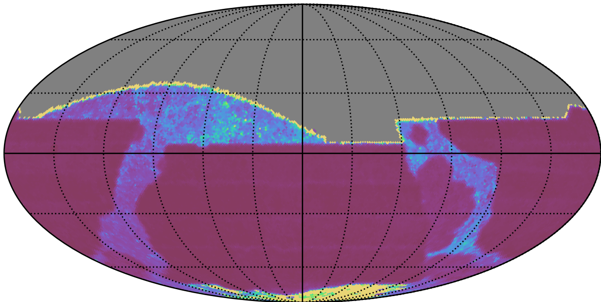
too_ignore_10_1v3.4_10yrs All sky z band: Median Inter-Night Gap
