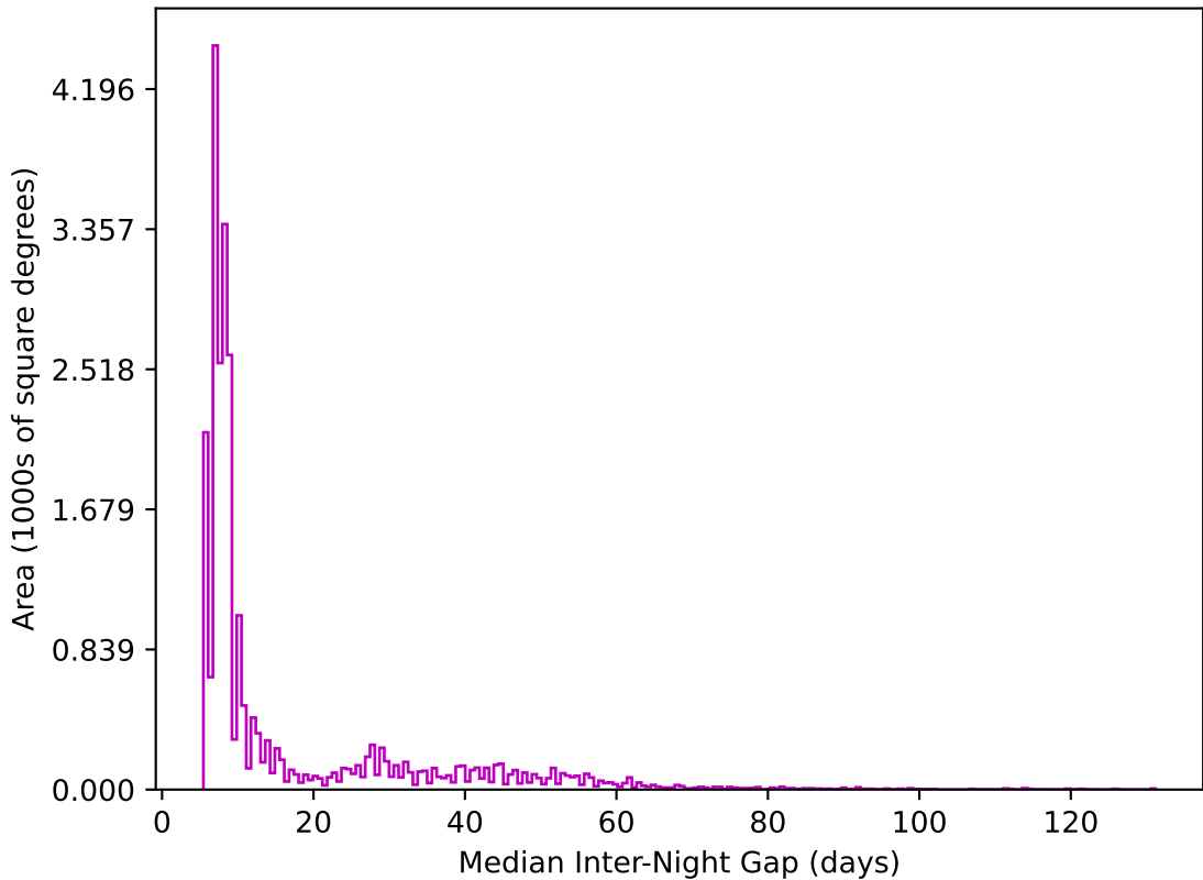
too_ignore_10_1v3.4_10yrs All sky z band: Median Inter-Night Gap
