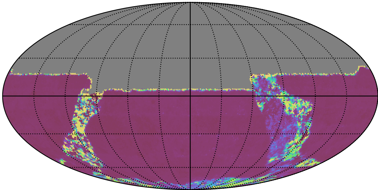
too_ignore_10_1v3.4_10yrs All sky u band: Median Inter-Night Gap
