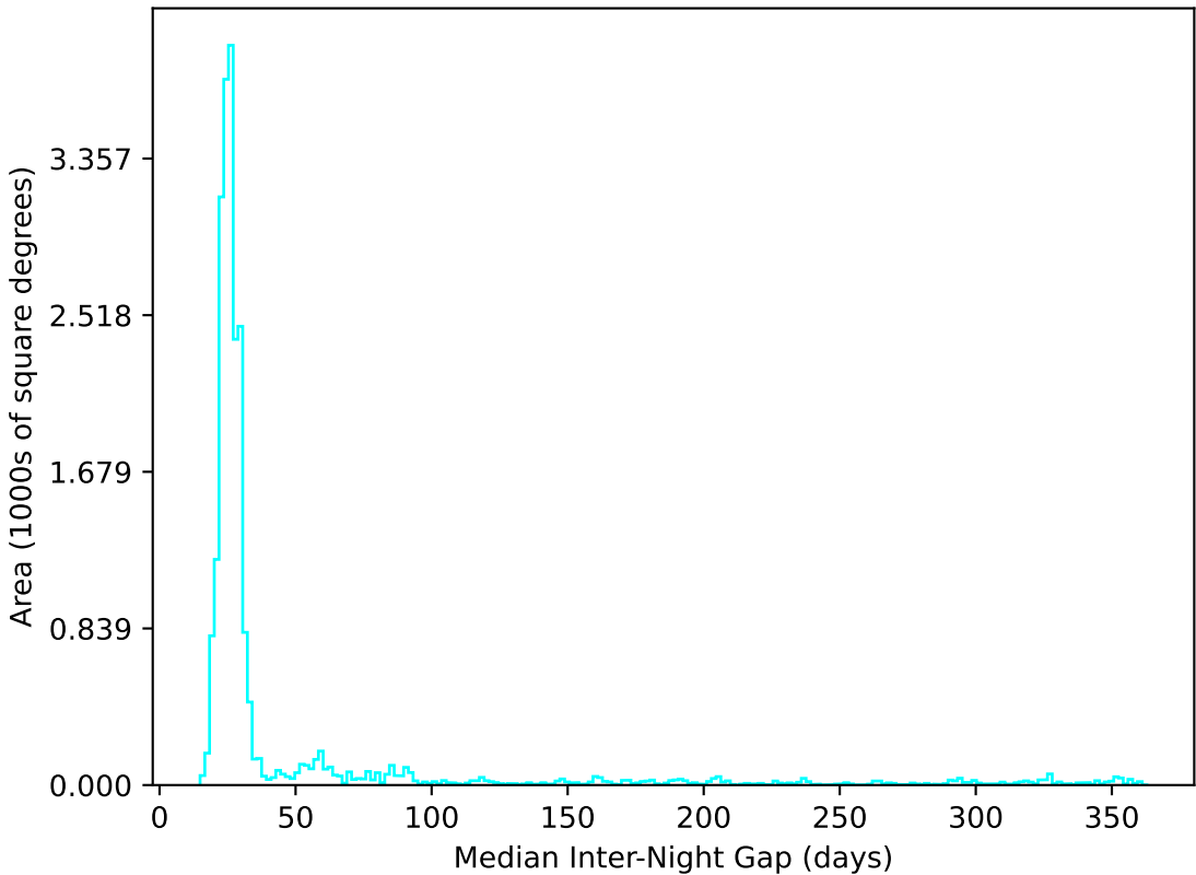
too_ignore_10_1v3.4_10yrs All sky u band: Median Inter-Night Gap
