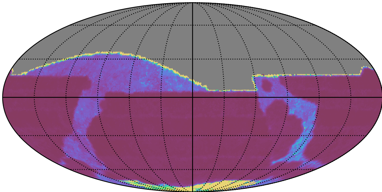
too_ignore_10_1v3.4_10yrs All sky r band: Median Inter-Night Gap
