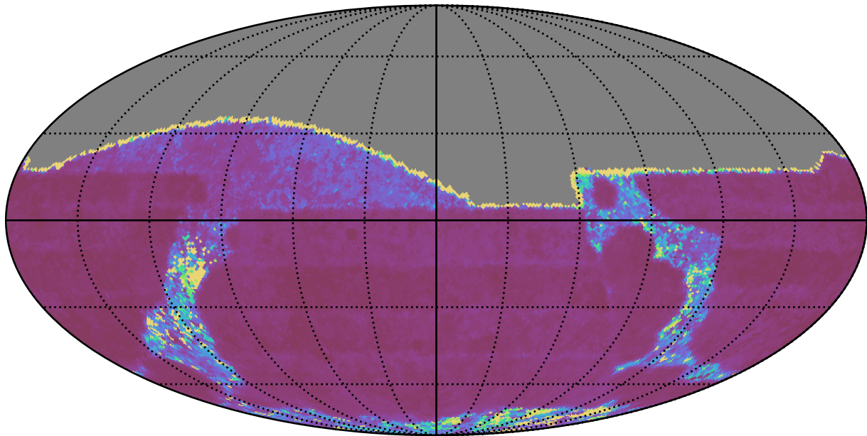
too_ignore_10_1v3.4_10yrs All sky g band: Median Inter-Night Gap
