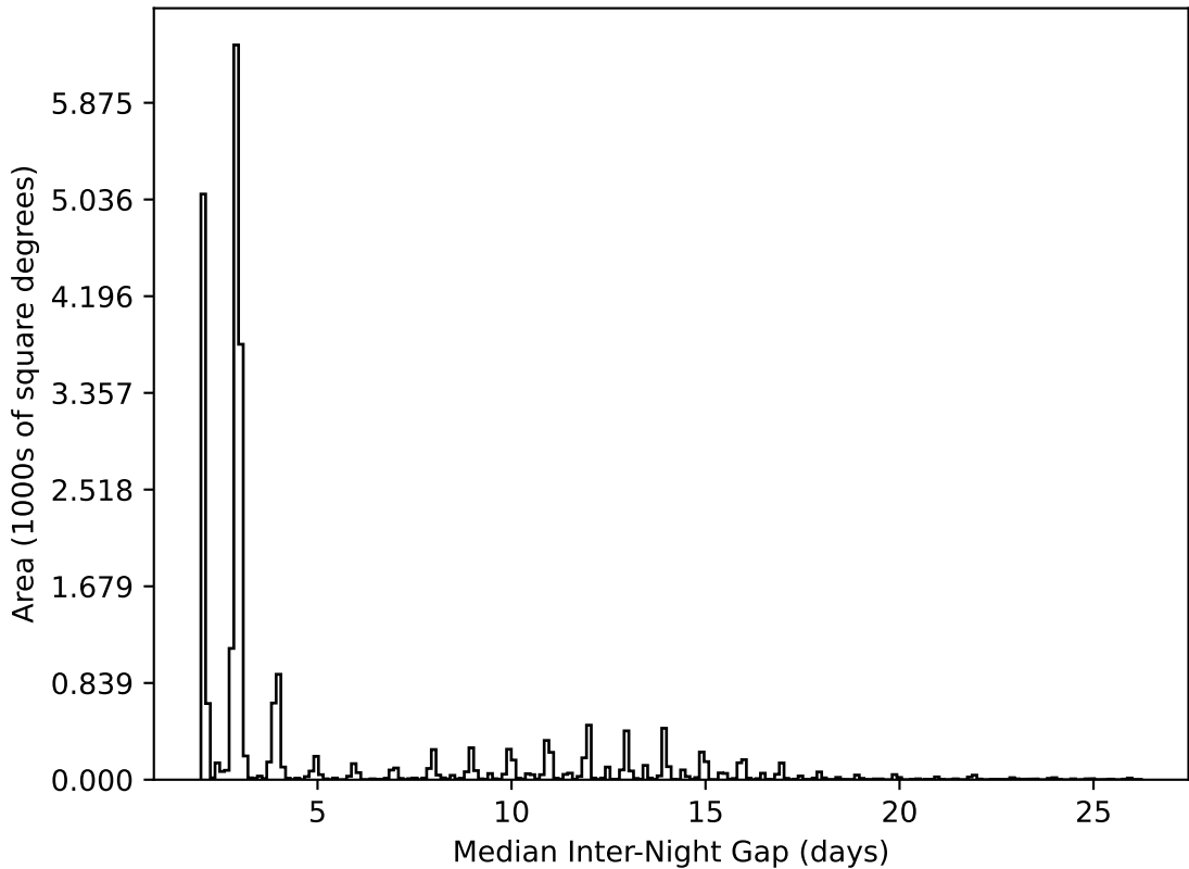
too_ignore_10_1v3.4_10yrs All sky all bands: Median Inter-Night Gap
