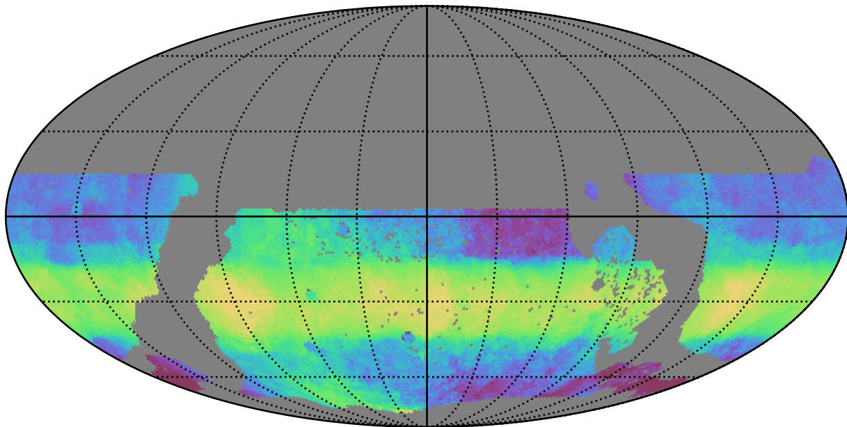
too_ignore_10_1v3.4_10yrs WFD z band: Median HA
