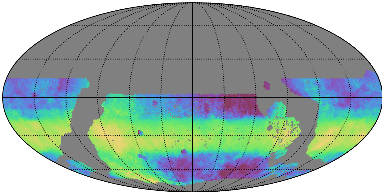
too_ignore_10_1v3.4_10yrs WFD y band: Median HA
