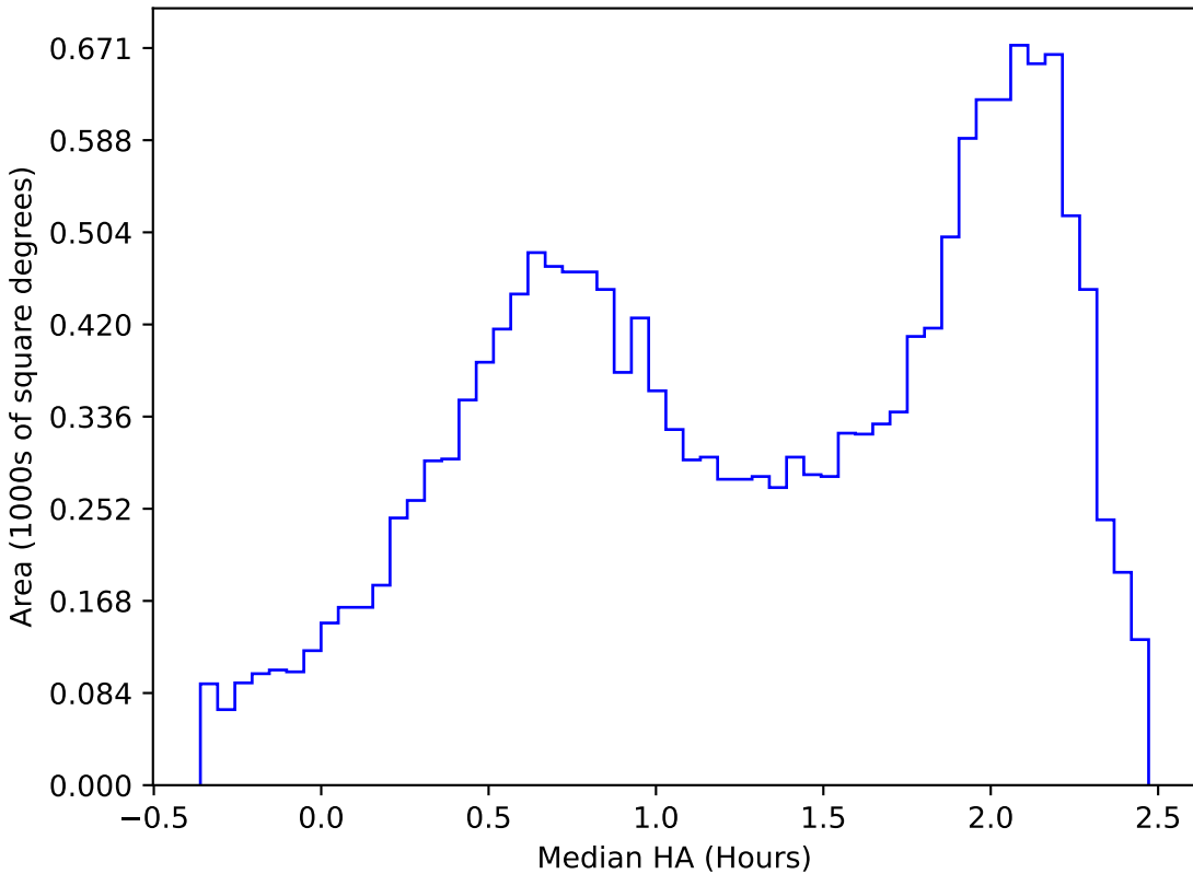
too_ignore_10_1v3.4_10yrs WFD y band: Median HA
