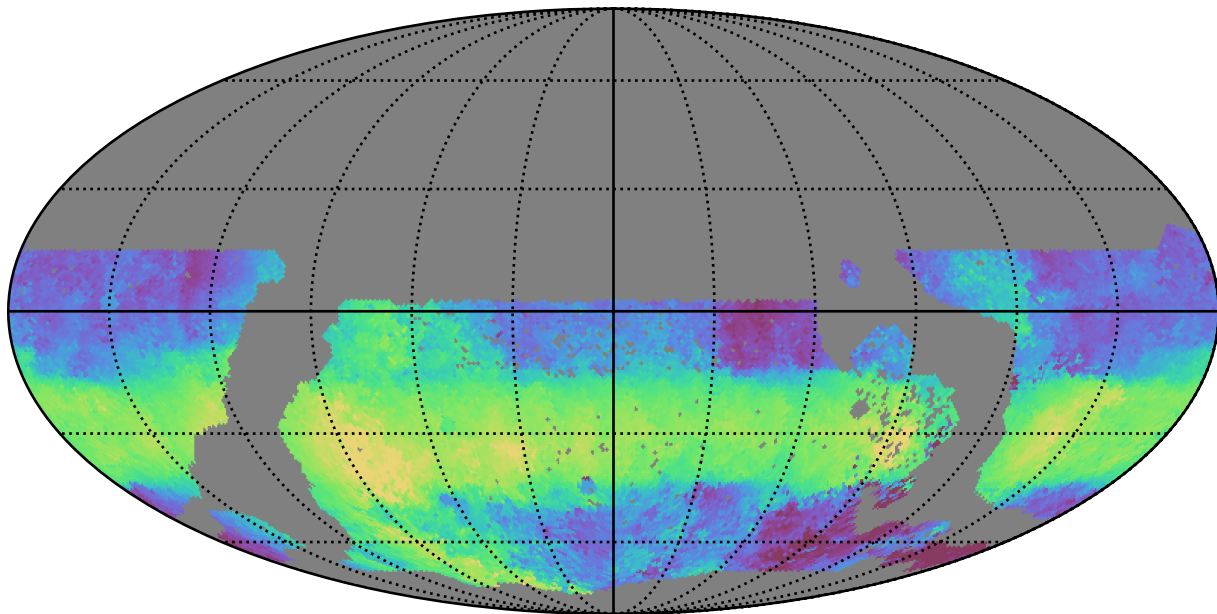
too_ignore_10_1v3.4_10yrs WFD u band: Median HA
