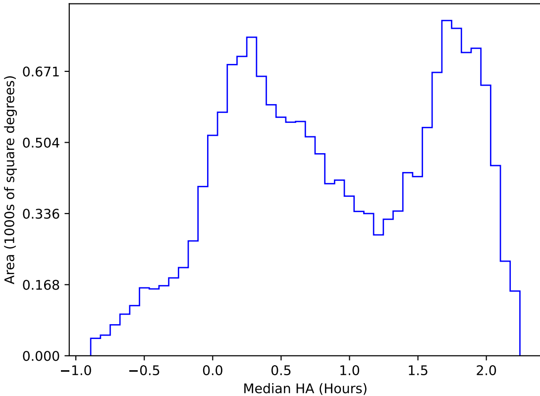
too_ignore_10_1v3.4_10yrs WFD r band: Median HA
