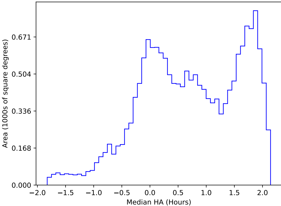
too_ignore_10_1v3.4_10yrs WFD g band: Median HA
