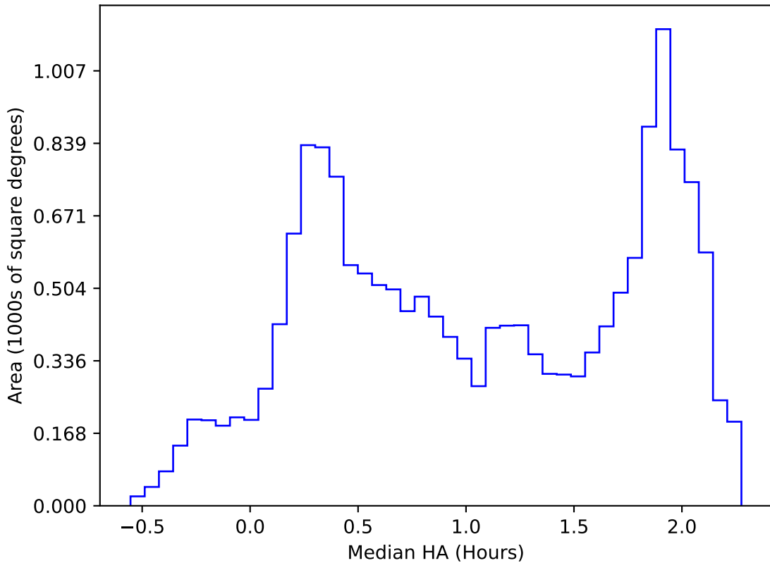
too_ignore_10_1v3.4_10yrs WFD all bands: Median HA
