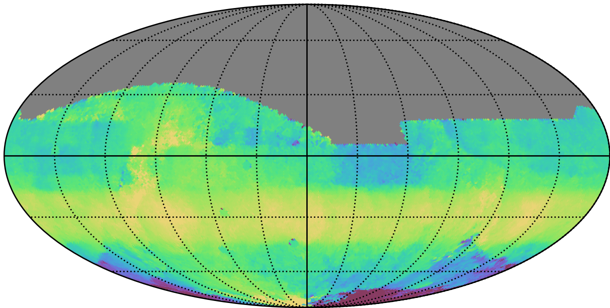
too_ignore_10_1v3.4_10yrs All sky z band: Median HA
