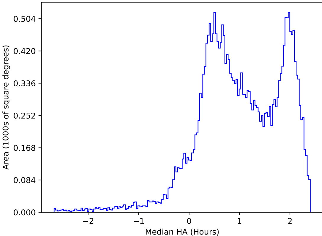
too_ignore_10_1v3.4_10yrs All sky z band: Median HA
