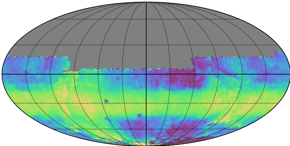
too_ignore_10_1v3.4_10yrs All sky y band: Median HA
