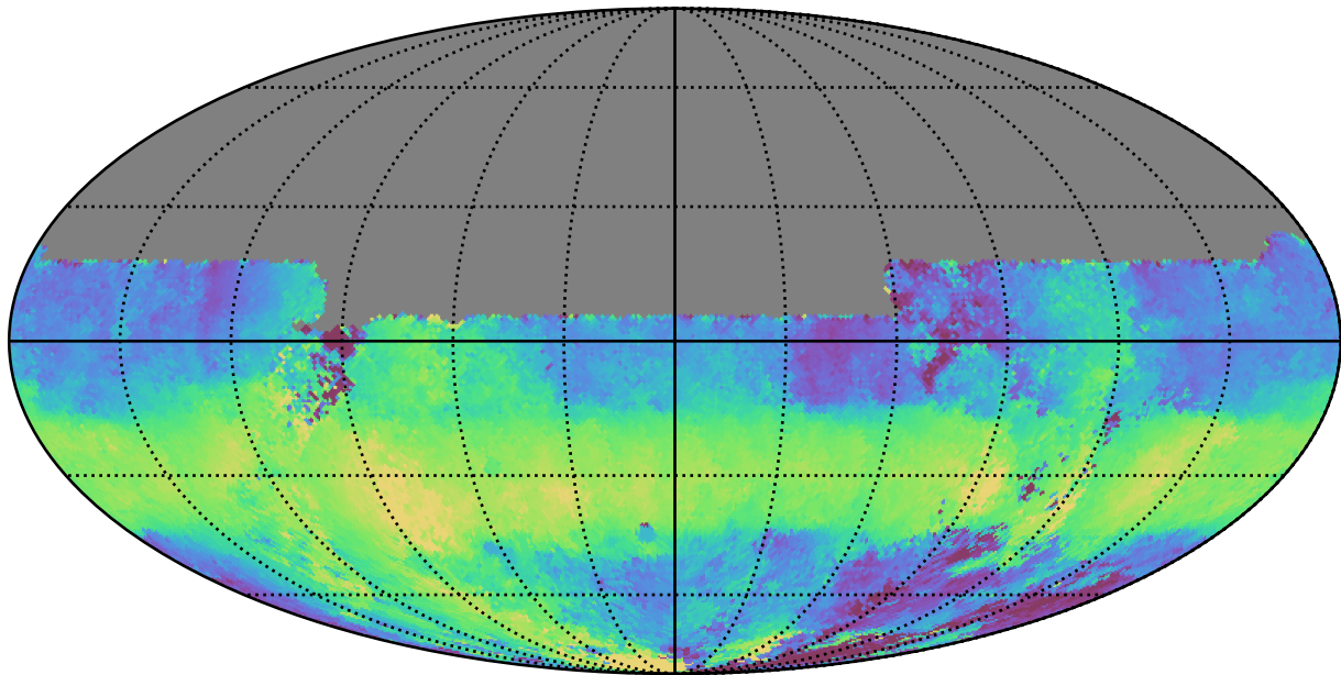
too_ignore_10_1v3.4_10yrs All sky u band: Median HA
