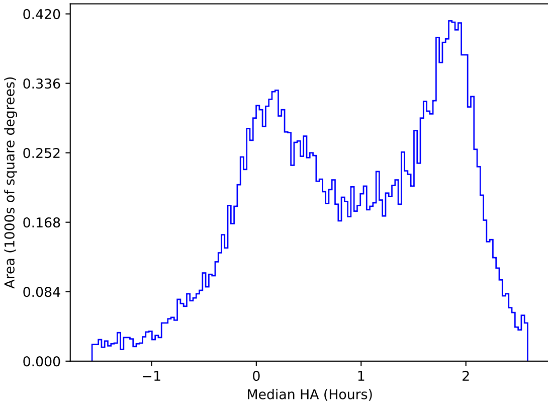
too_ignore_10_1v3.4_10yrs All sky u band: Median HA
