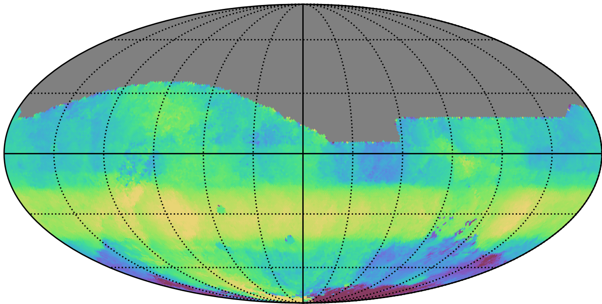
too_ignore_10_1v3.4_10yrs All sky r band: Median HA
