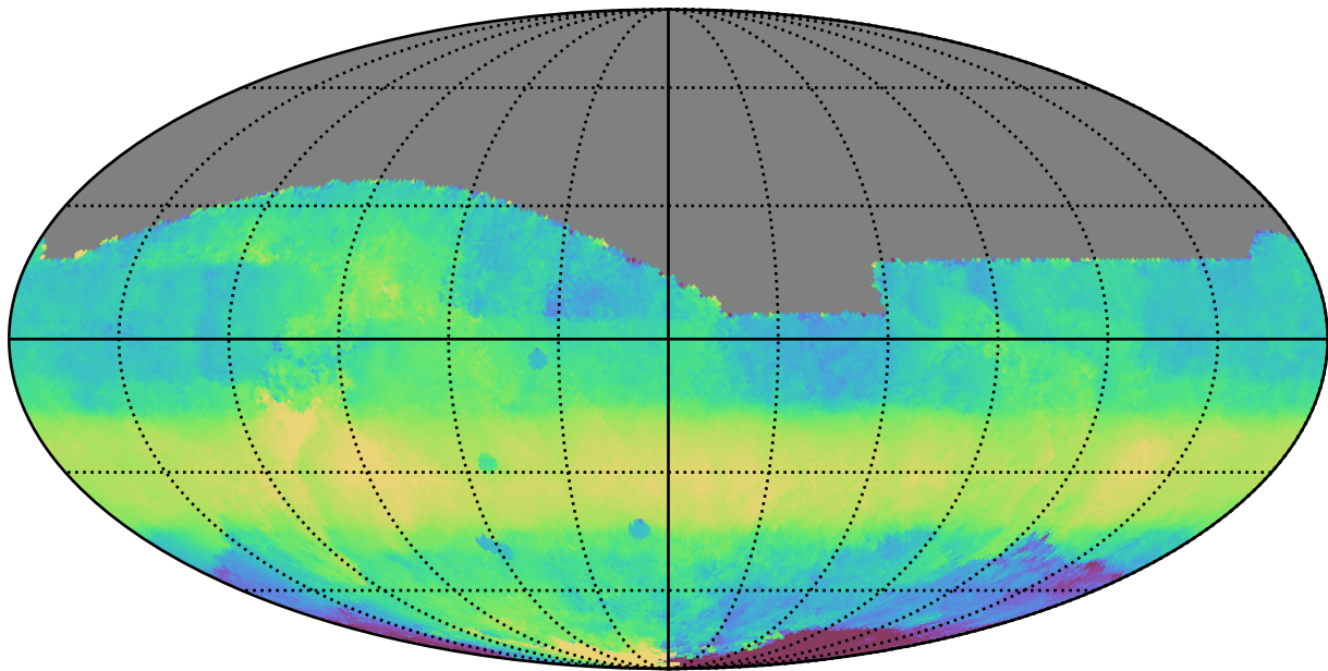
too_ignore_10_1v3.4_10yrs All sky i band: Median HA
