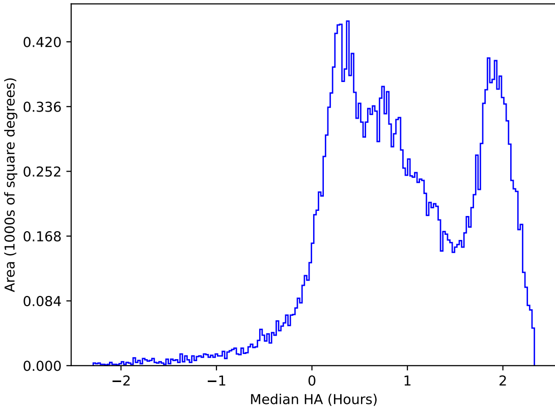
too_ignore_10_1v3.4_10yrs All sky i band: Median HA
