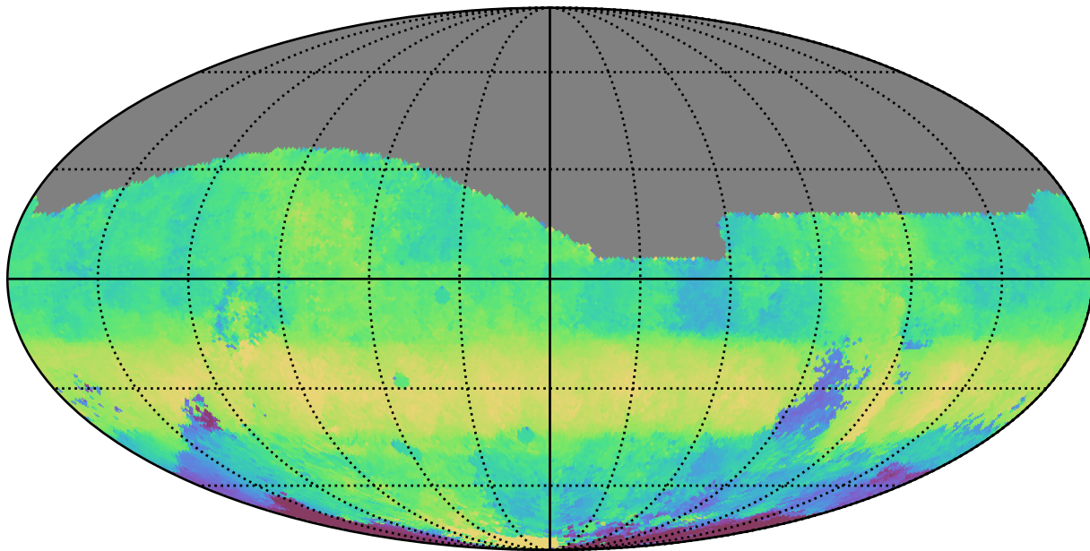
too_ignore_10_1v3.4_10yrs All sky g band: Median HA
