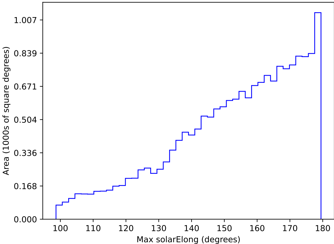
too_ignore_10_1v3.4_10yrs WFD z band: Max solarElong
