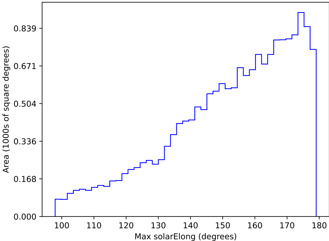
too_ignore_10_1v3.4_10yrs WFD u band: Max solarElong
