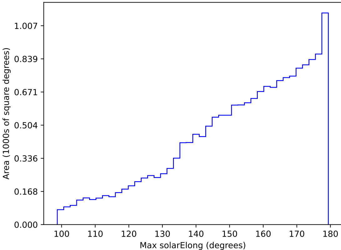
too_ignore_10_1v3.4_10yrs WFD r band: Max solarElong
