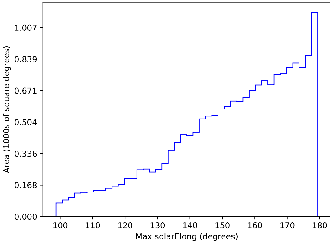
too_ignore_10_1v3.4_10yrs WFD i band: Max solarElong
