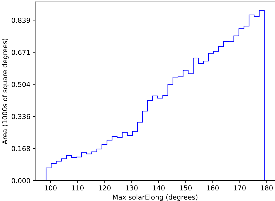
too_ignore_10_1v3.4_10yrs WFD g band: Max solarElong
