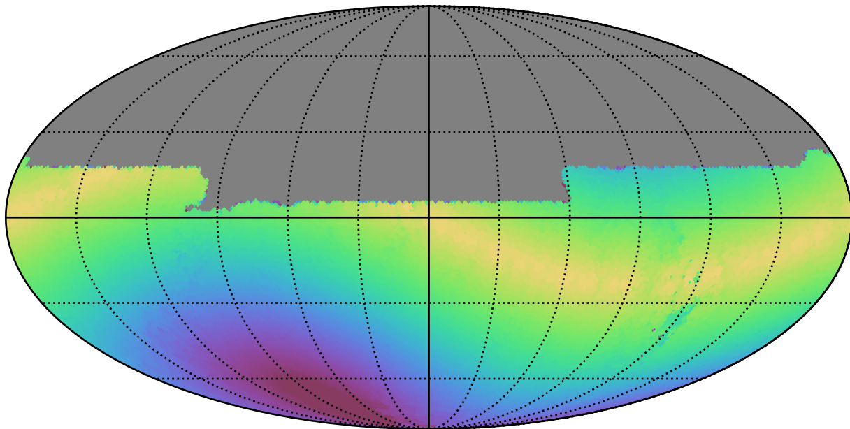
too_ignore_10_1v3.4_10yrs All sky u band: Max solarElong
