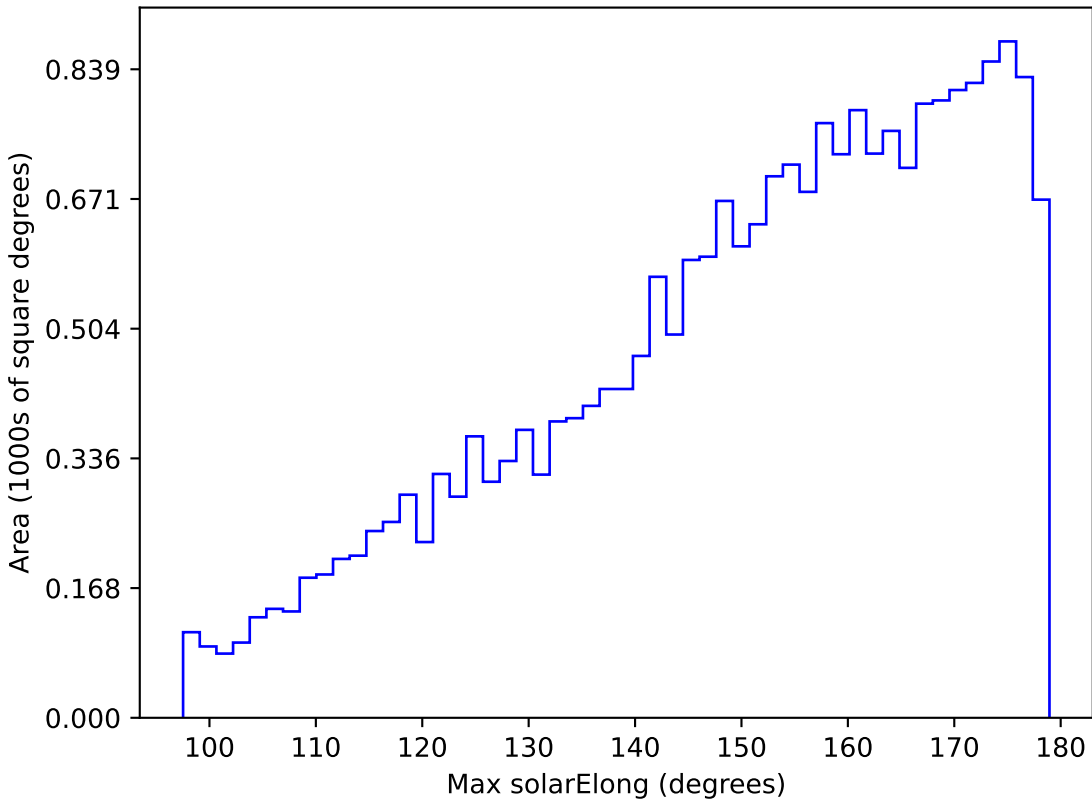
too_ignore_10_1v3.4_10yrs All sky u band: Max solarElong
