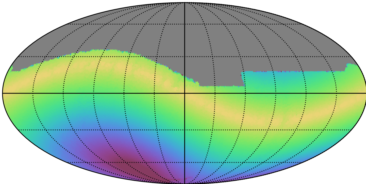
too_ignore_10_1v3.4_10yrs All sky r band: Max solarElong
