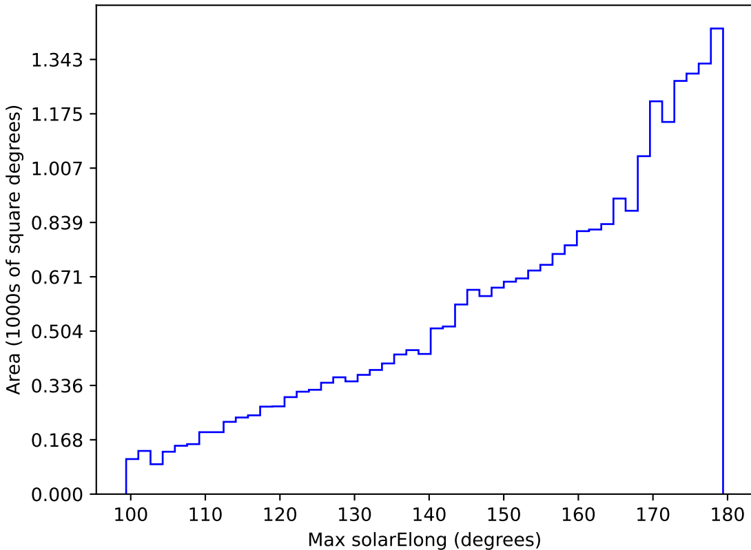
too_ignore_10_1v3.4_10yrs All sky r band: Max solarElong
