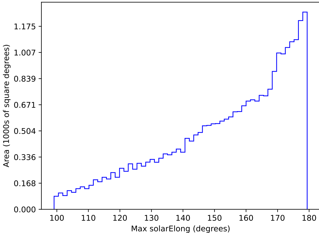
too_ignore_10_1v3.4_10yrs All sky i band: Max solarElong
