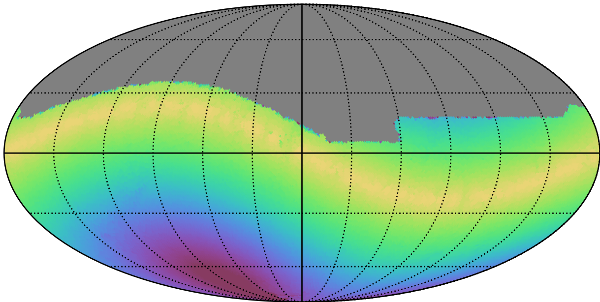
too_ignore_10_1v3.4_10yrs All sky g band: Max solarElong
