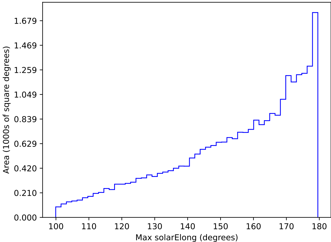
too_ignore_10_1v3.4_10yrs All sky all bands: Max solarElong
