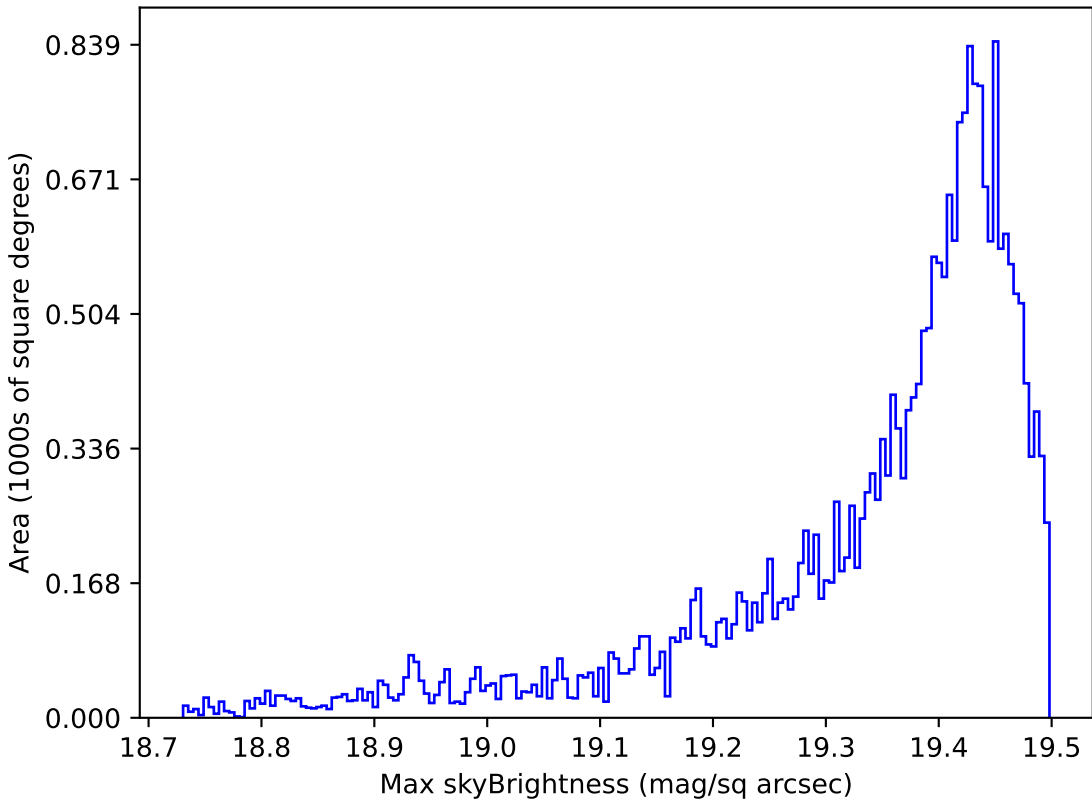
too_ignore_10_1v3.4_10yrs Yr 1 z band: Max skyBrightness
