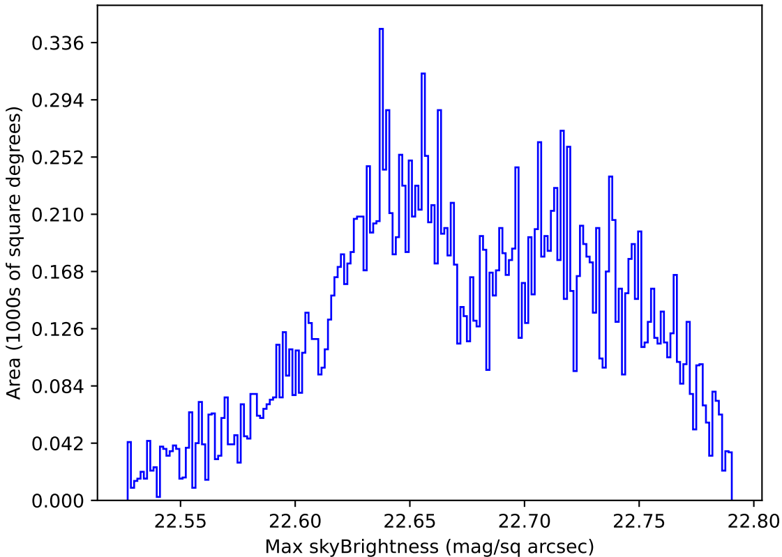
too_ignore_10_1v3.4_10yrs Yr 1 u band: Max skyBrightness
