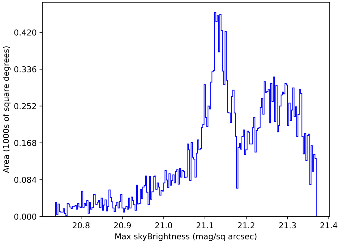
too_ignore_10_1v3.4_10yrs Yr 1 r band: Max skyBrightness
