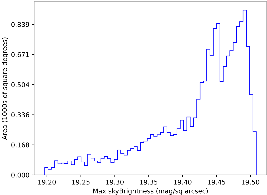
too_ignore_10_1v3.4_10yrs WFD z band: Max skyBrightness
