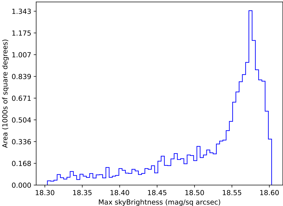
too_ignore_10_1v3.4_10yrs WFD y band: Max skyBrightness
